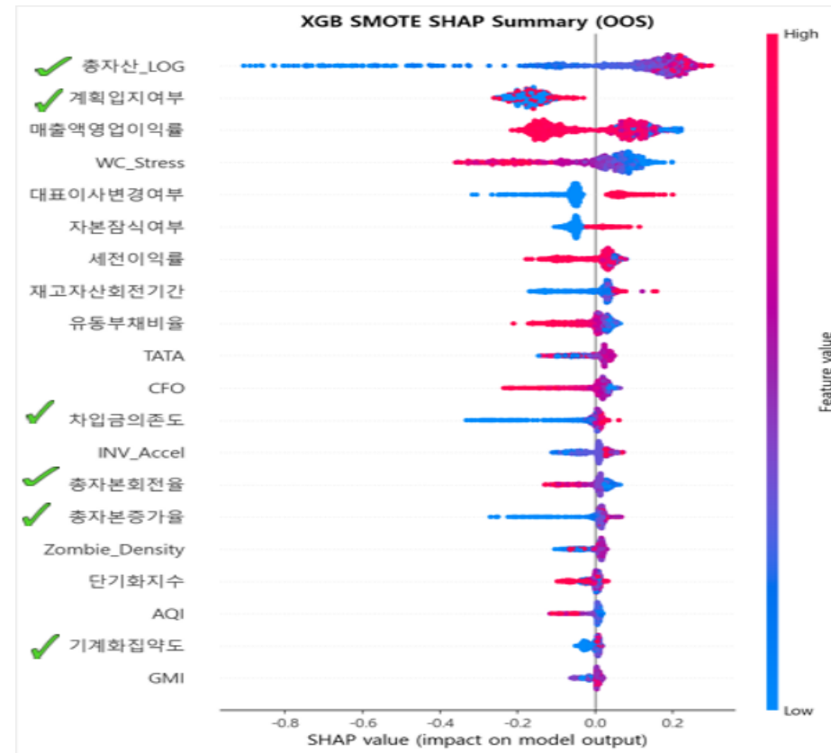
XGB SMOTE SHAP Summary Plot (OOS 기준)
